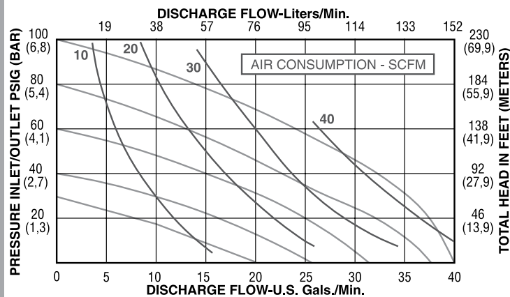
PERFORMANCE CURVE
