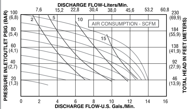
PERFORMANCE CURVE
