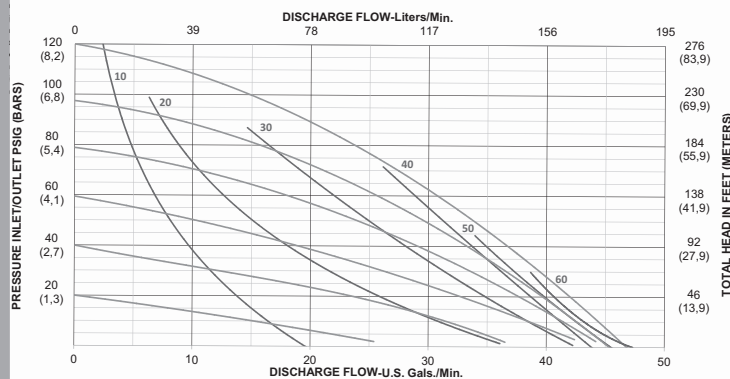
PERFORMANCE CURVE (1" TPE)*
