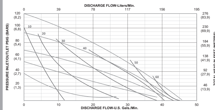
PERFORMANCE CURVE (1" PTFE)*
