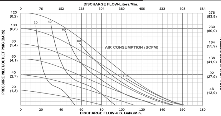
PERFORMANCE CURVE (2" TPE)
