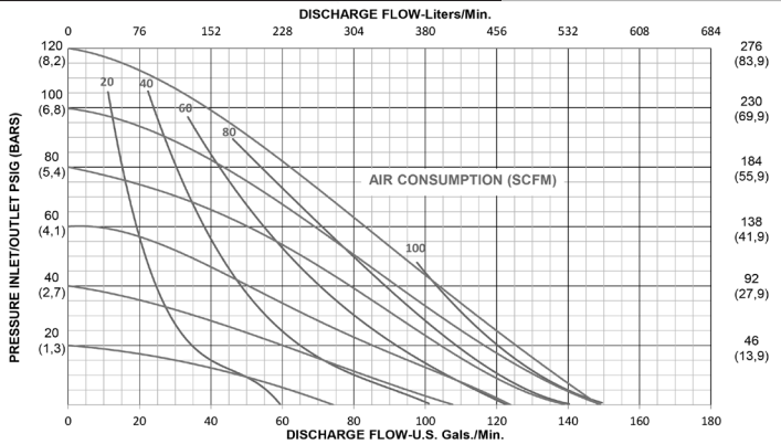
PERFORMANCE CURVE (2" PTFE)
