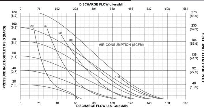
PERFORMANCE CURVE (2" RUBBER)
