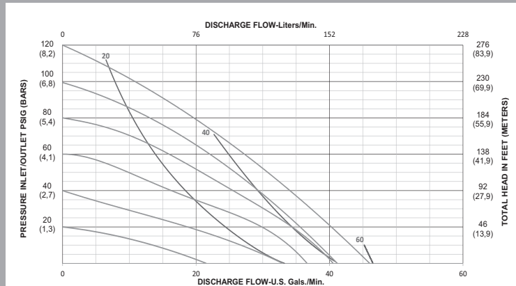
PERFORMANCE CURVE (1" RUBBER)*
