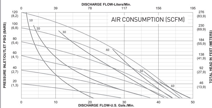
PERFORMANCE CURVE (1" RUBBER)*
