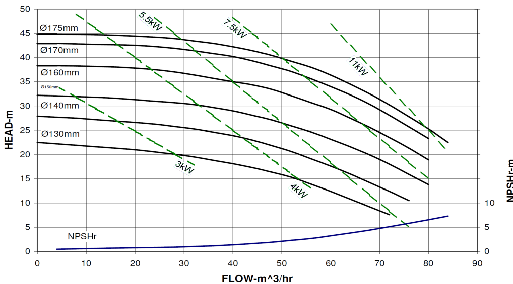
LM-V532 2900 RPM
