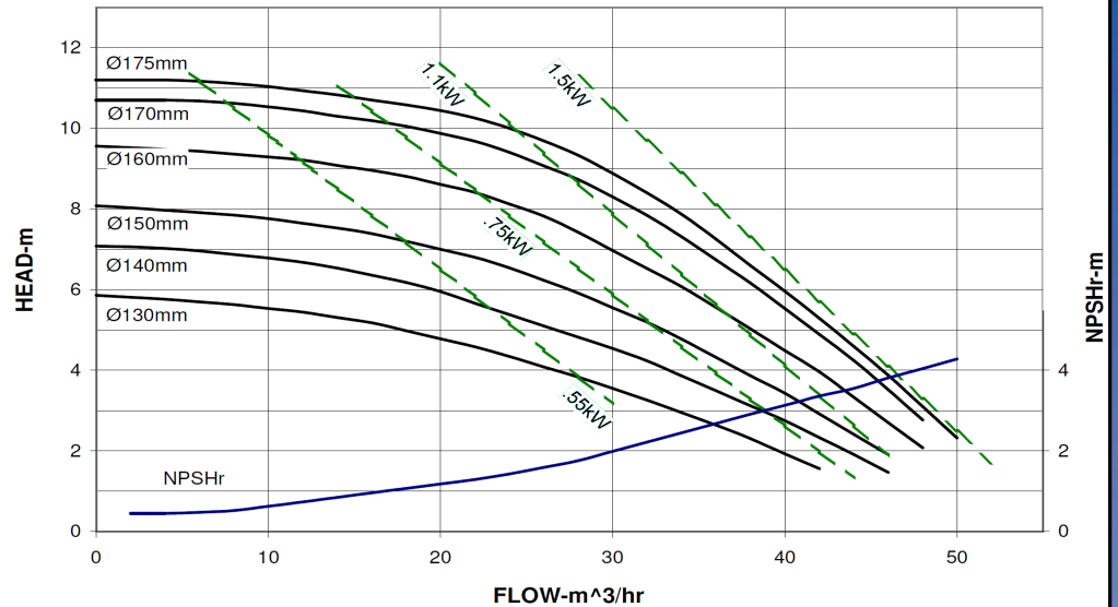
LM-V531 1450 RPM
