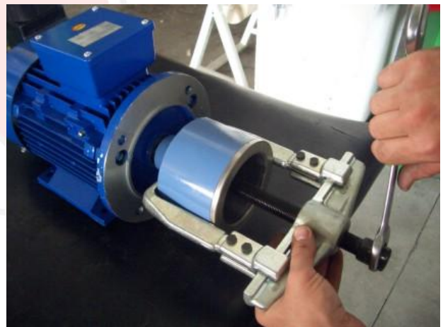
13) Using an extractor pull-out the external magnet from motor shaft.
